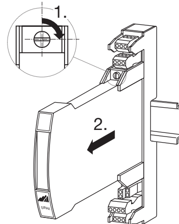
Fig. 9. Withdraw the module from the base.
