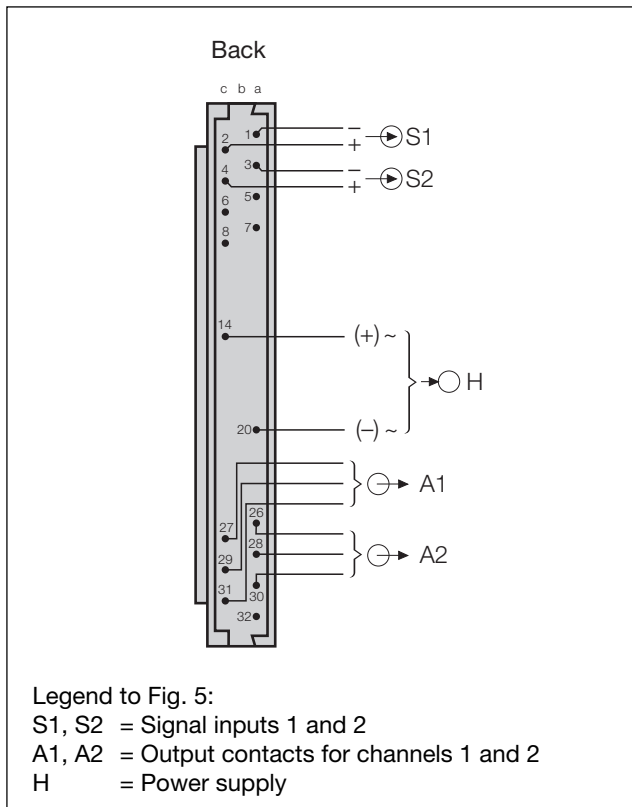
Fig. 5. Plug arrangement seen from the rear of SIRAX SV 824.
